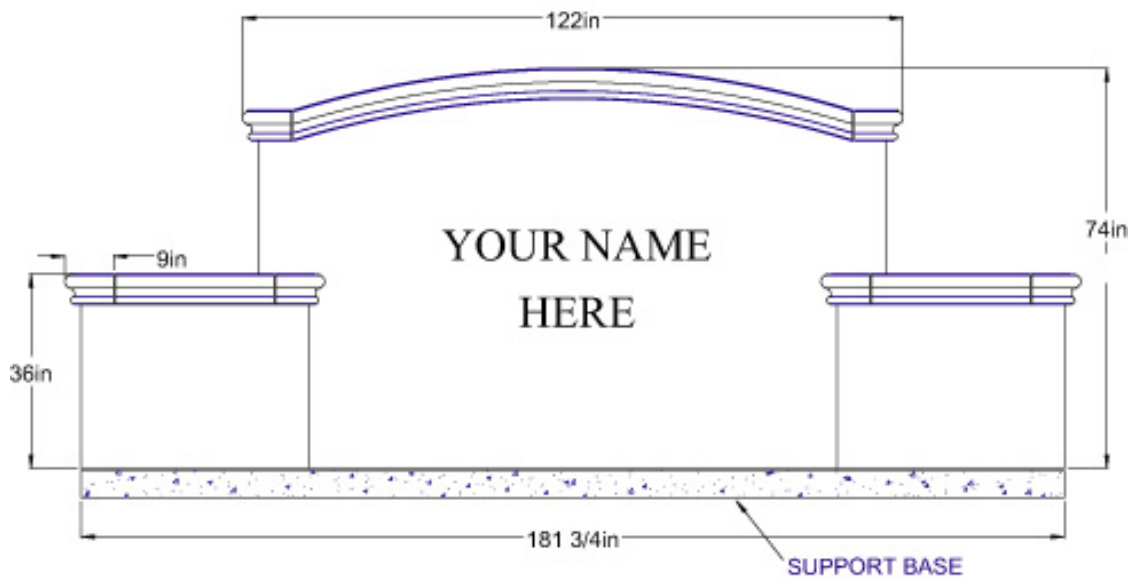
ELEVATION VIEW
